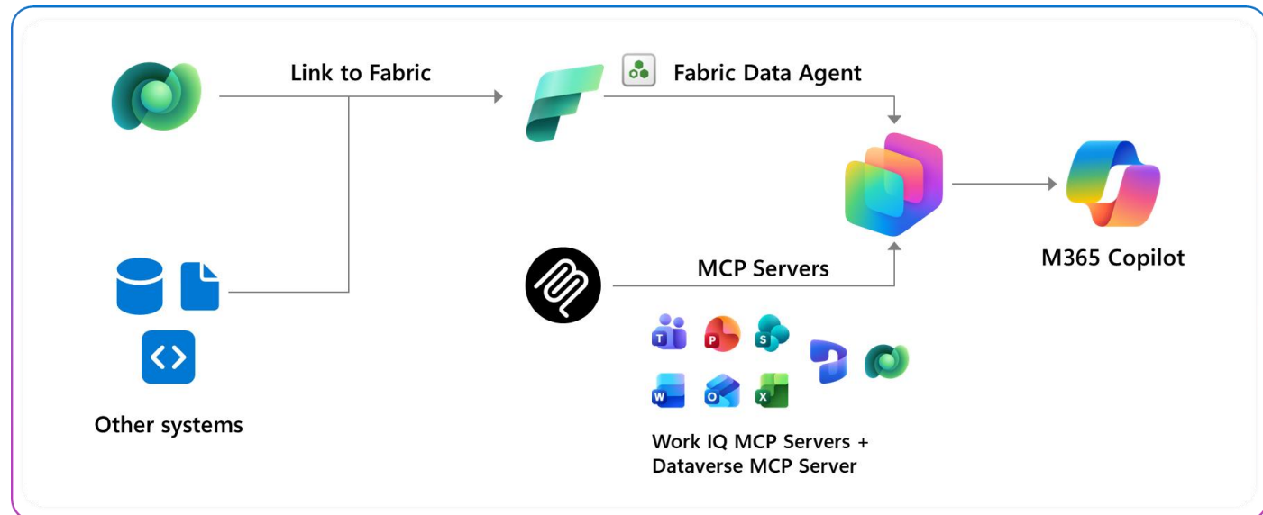
Pattern 2b: Real time + analytical workflows
