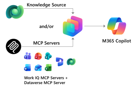
Pattern 1: Real-time workflows
