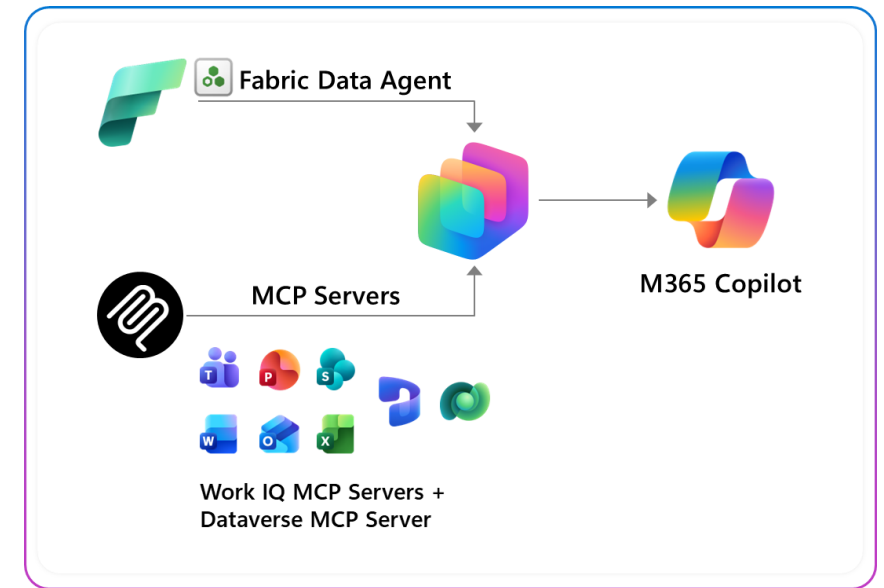
Pattern 2a: Real time + analytical workflows
