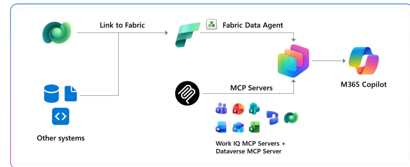
Pattern 2b: Real time + analytical workflows
